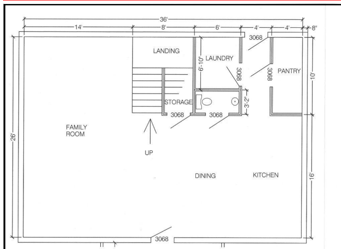
First floor includes space for kitchen, dining and living room. (plans prepared by Aaron Reed)
