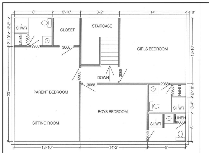
Second floor will have bedrooms for house parents and twelve children.
